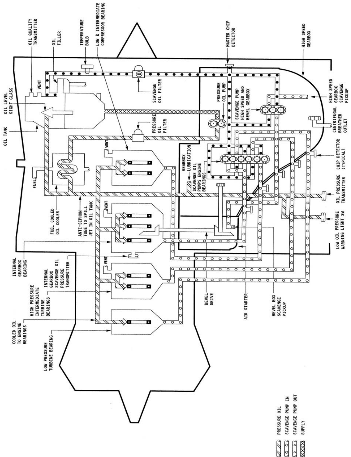
RB211 Engine Oil System Schematic
